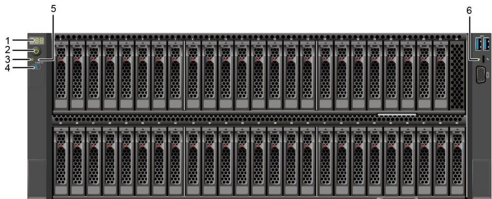
Figure 5-14 Indicators and buttons on the front panel
