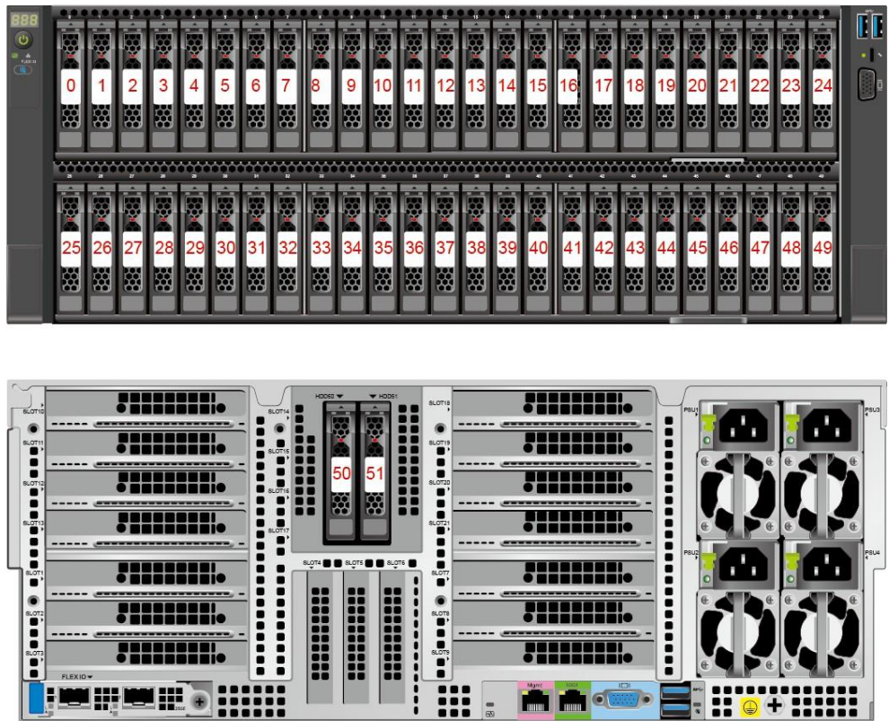
Figure 5-47 Drive numbering
