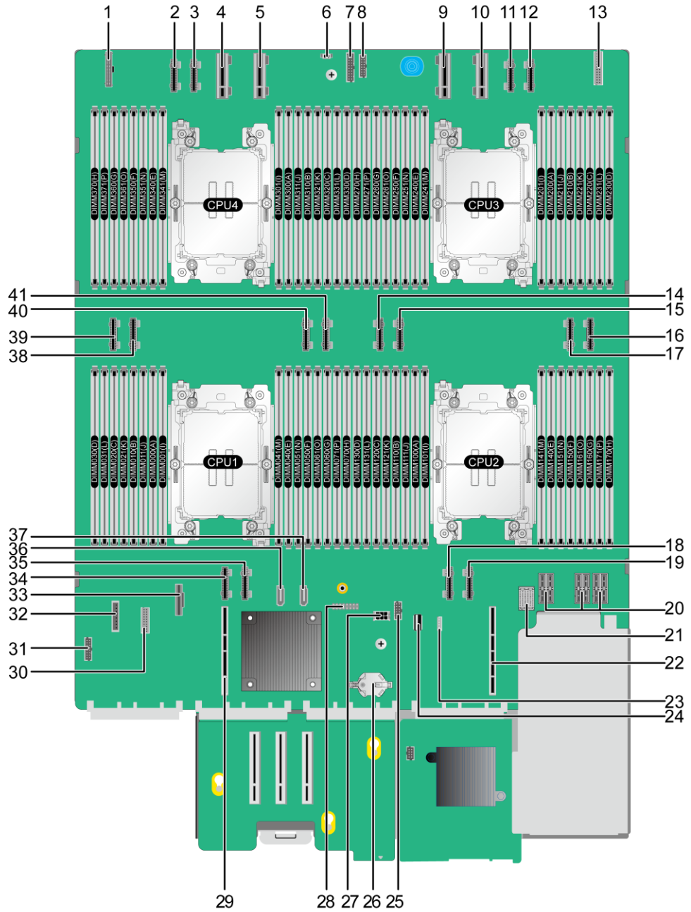
Figure 5-66 Mainboard
