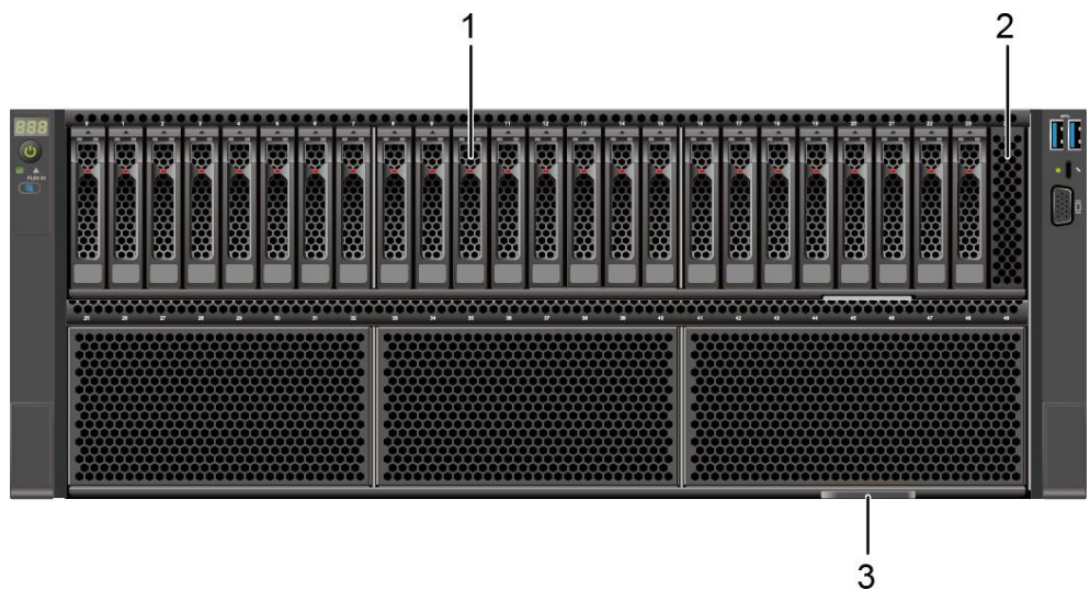
Figure 5-3 Front view
