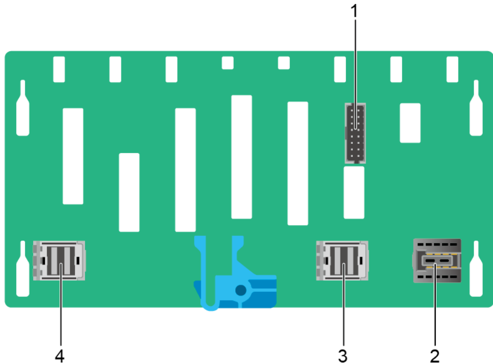
Figure 5-67 8 x 2.5" drive pass-through backplane
