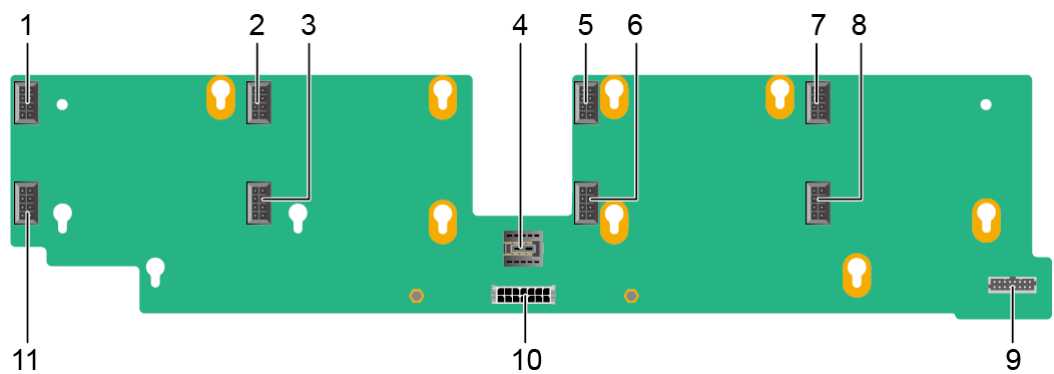
Figure 5-75 Fan board 1
