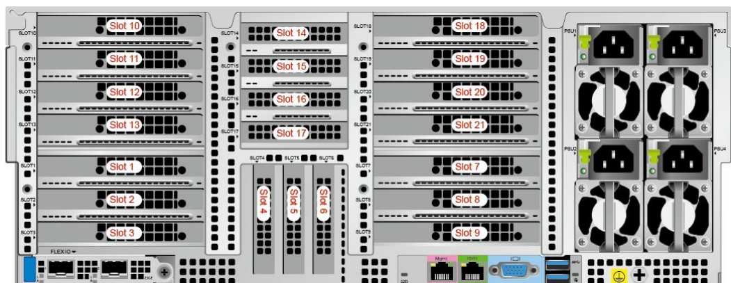
Figure 5-51 PCIe slots
