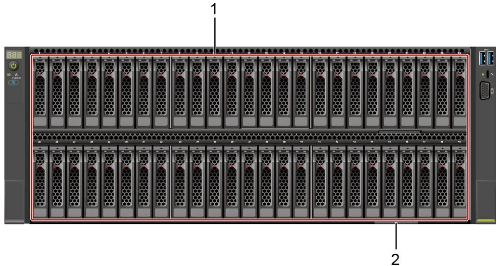
Figure 5-7 Front view
