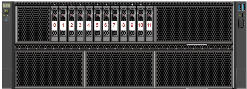
Figure 5-37 Drive numbering
