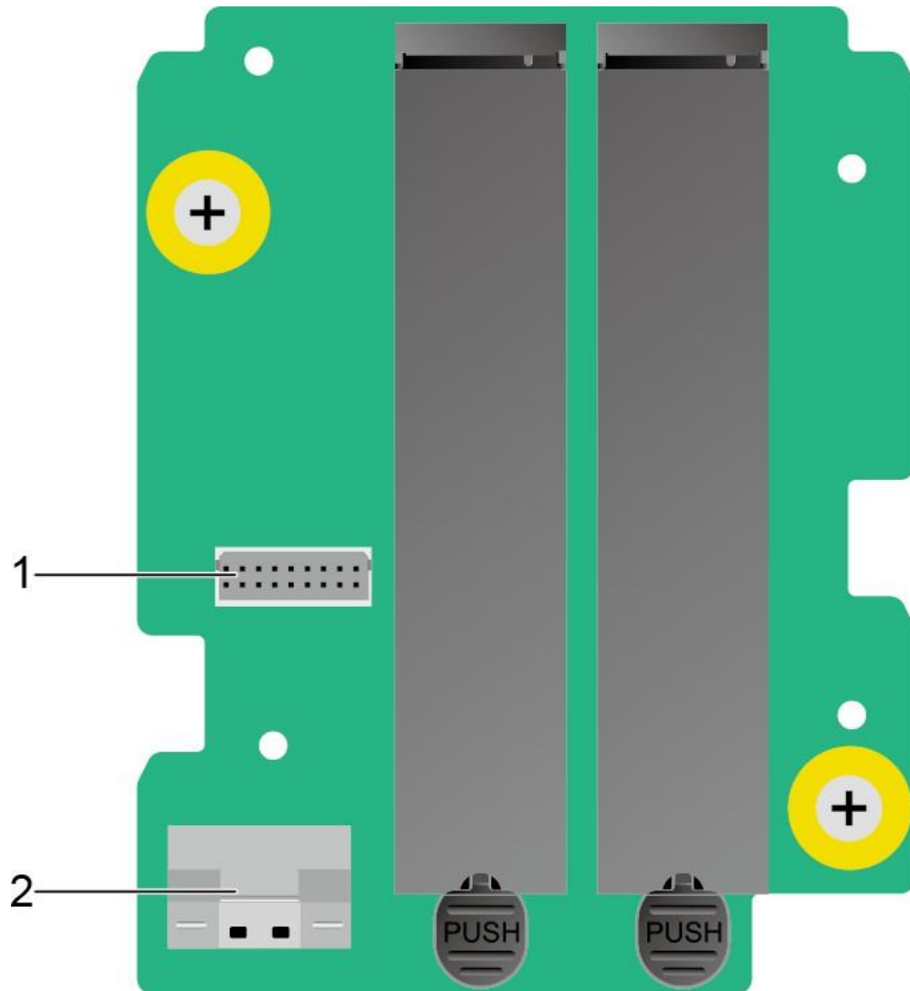
Figure 5-76 M.2 SSD adapter board
