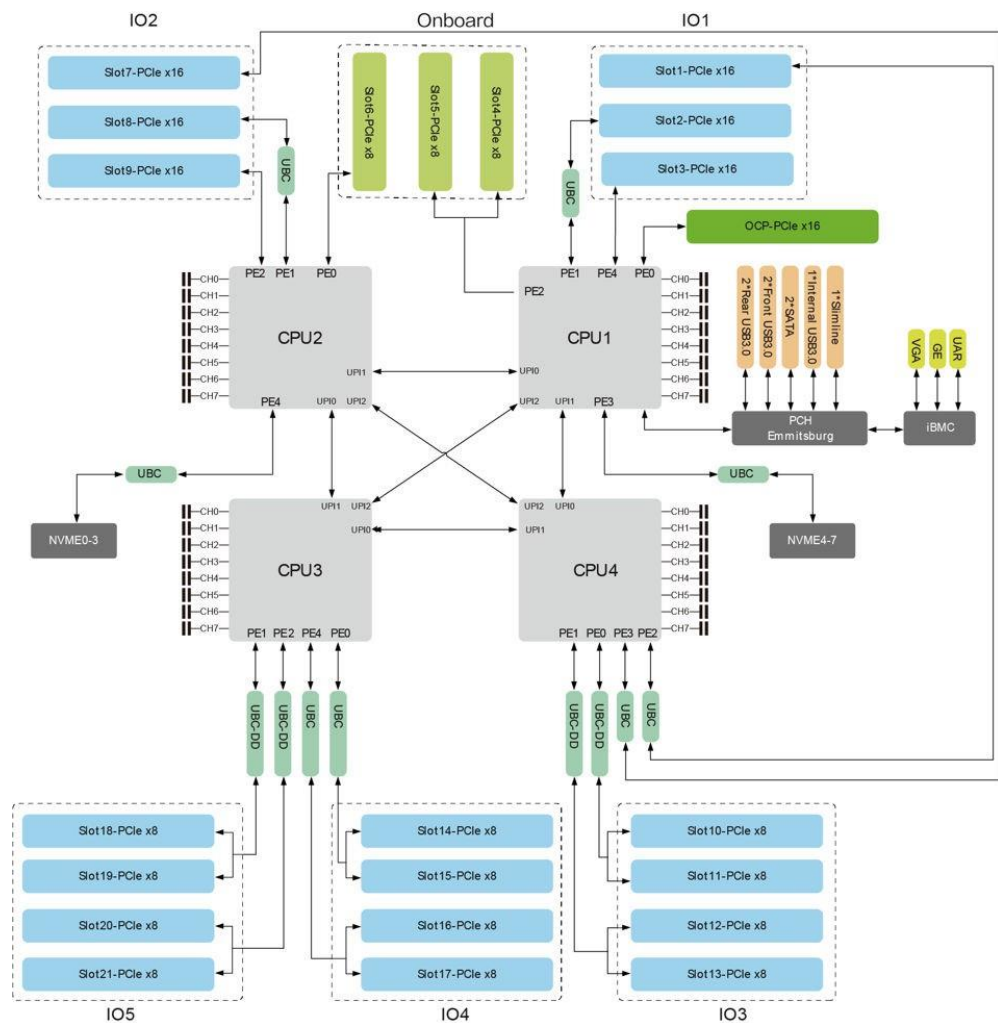
Figure 4-1 Logic structure
