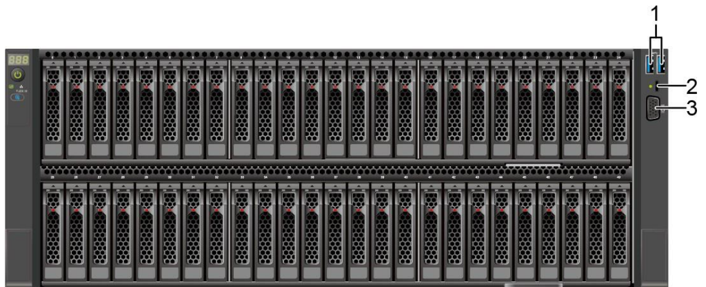
Figure 5-20 Ports on the front panel
