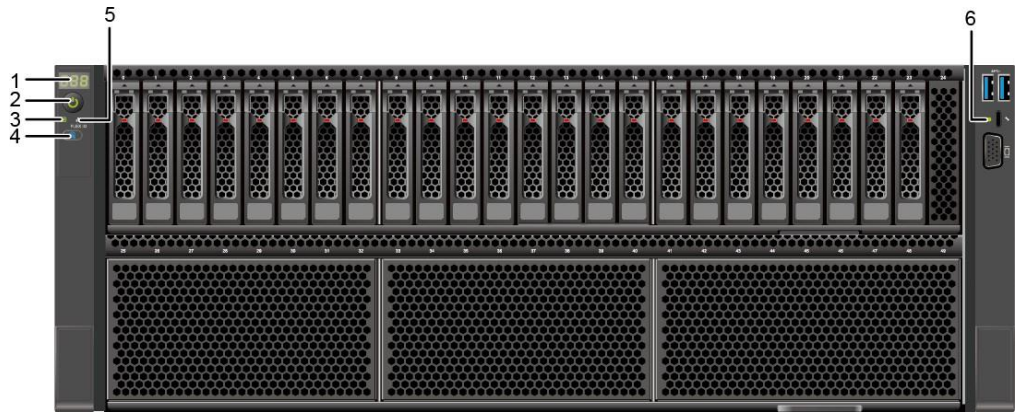
Figure 5-11 Indicators and buttons on the front panel
