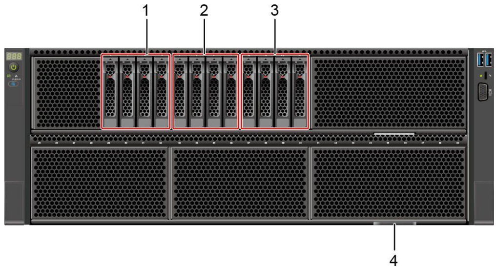
Figure 5-2 Front view
