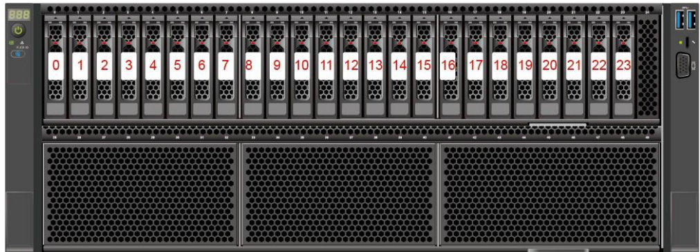
Figure 5-43 Drive numbering
