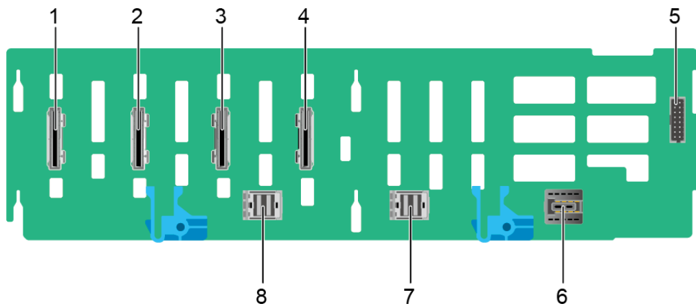
Figure 5-68 12 x 2.5" drive pass-through backplane
