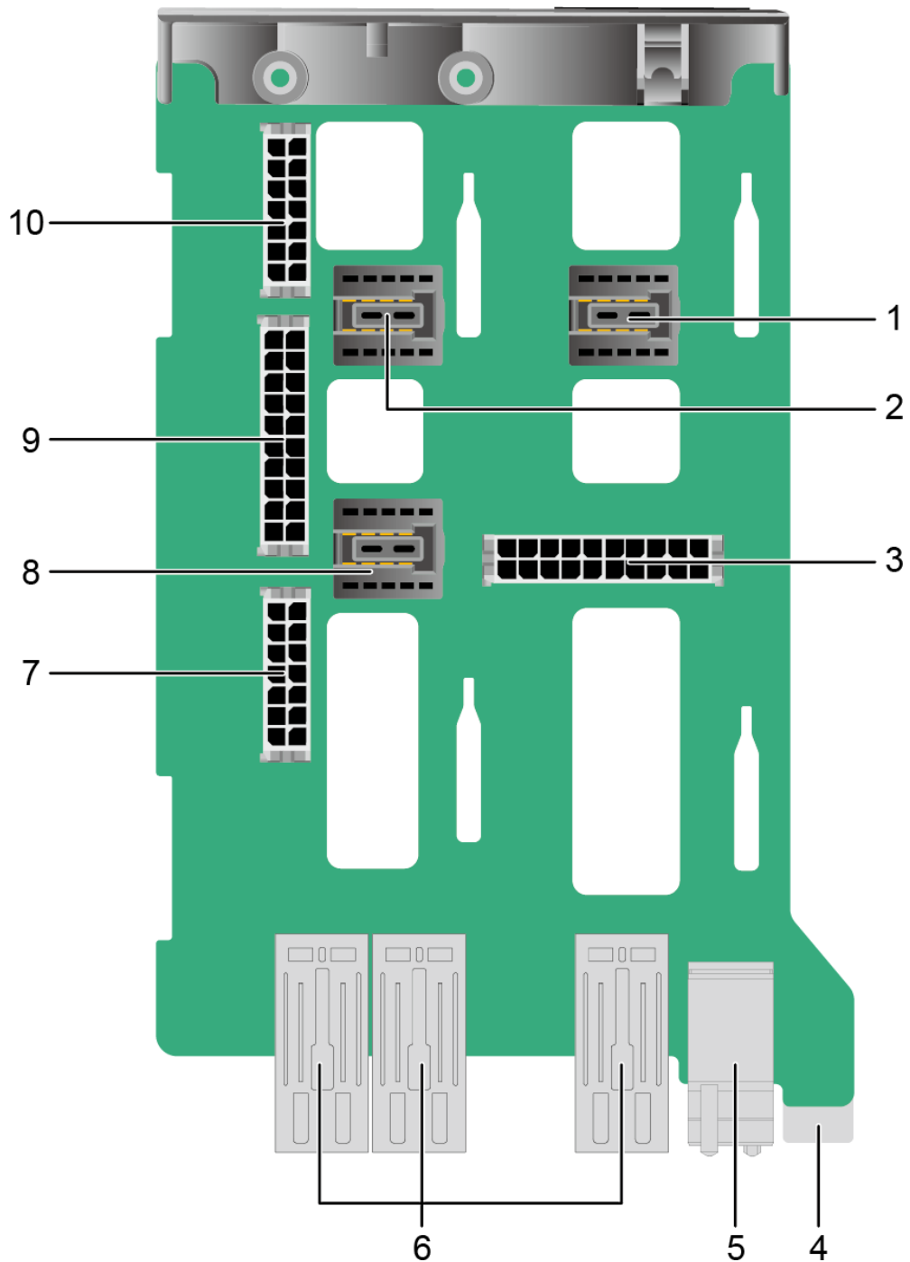
Figure 5-74 PSU backplane
