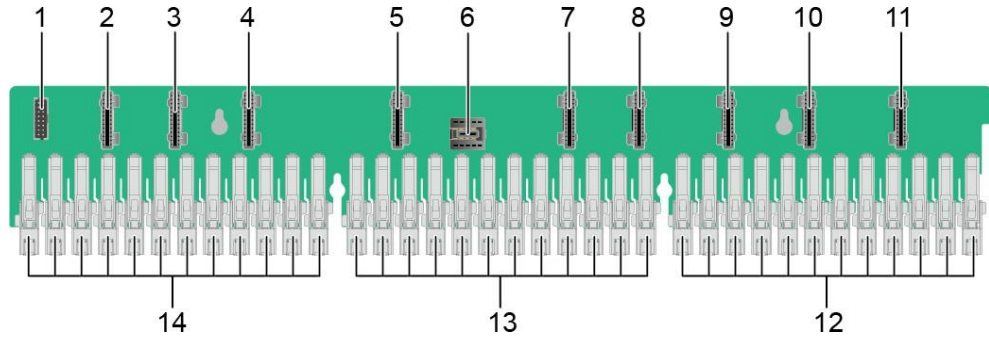
Figure 5-72 E1.S drive pass-through backplane
