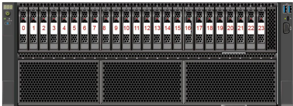
Figure 5-45 Drive numbering
