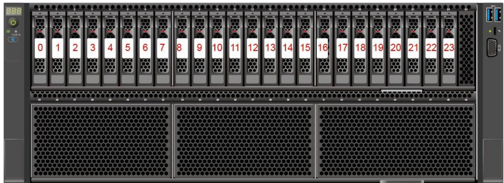
Figure 5-44 Drive numbering
