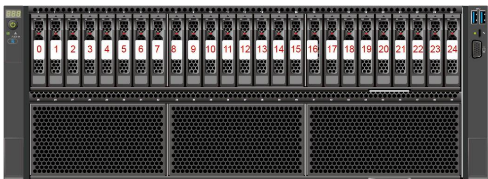
Figure 5-46 Drive numbering
