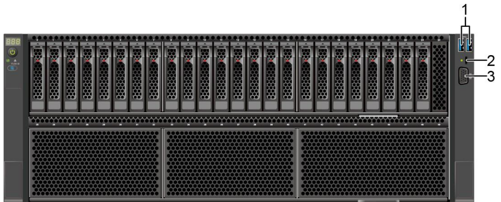
Figure 5-18 Ports on the front panel
