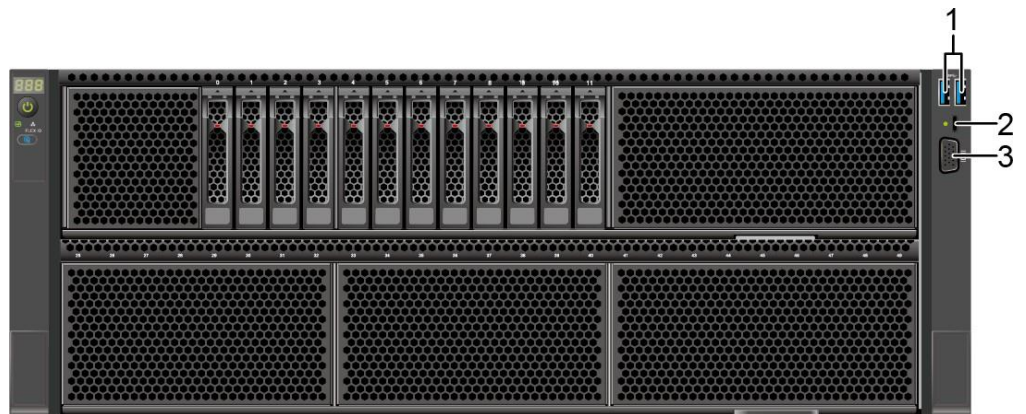
Figure 5-16 Ports on the front panel
