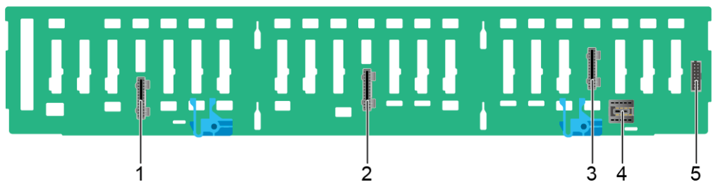
Figure 5-69 24 x 2.5" drive pass-through backplane
