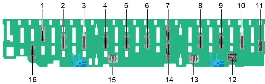
Figure 5-70 24 x 2.5" drive NVMe backplane
