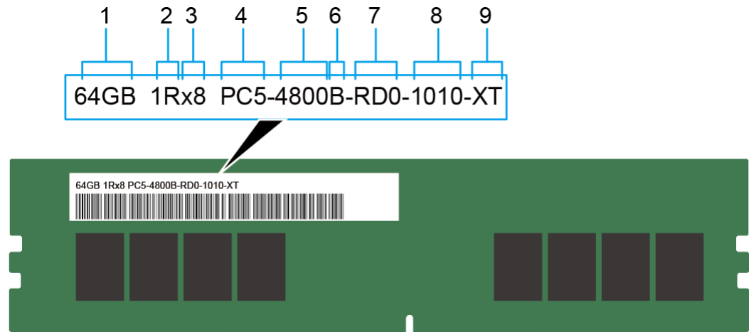
Figure 5-29 Memory identifier
