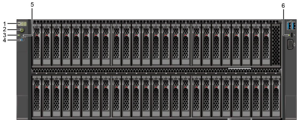
Figure 5-13 Indicators and buttons on the front panel
