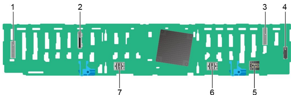
Figure 5-71 25 x 2.5" drive EXP backplane
