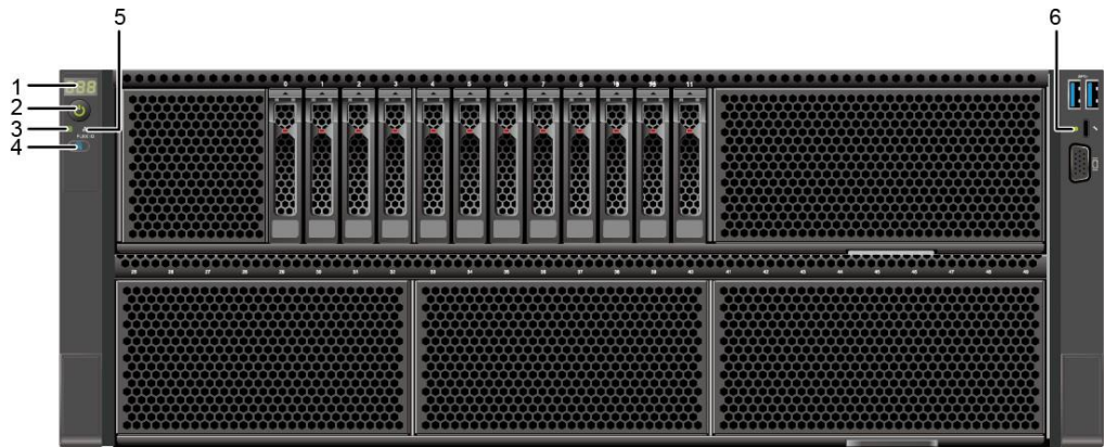
Figure 5-9 Indicators and buttons on the front panel
