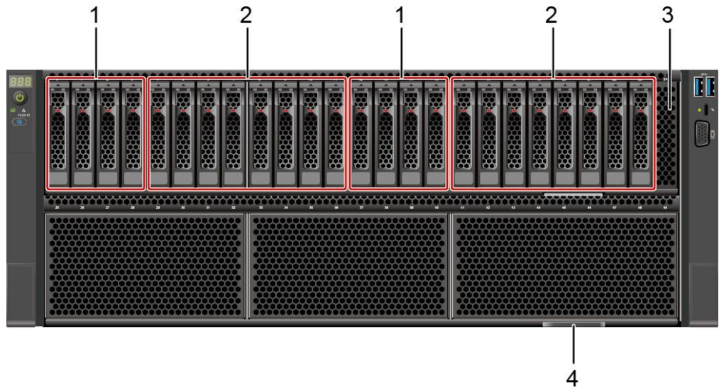
Figure 5-5 Front view
