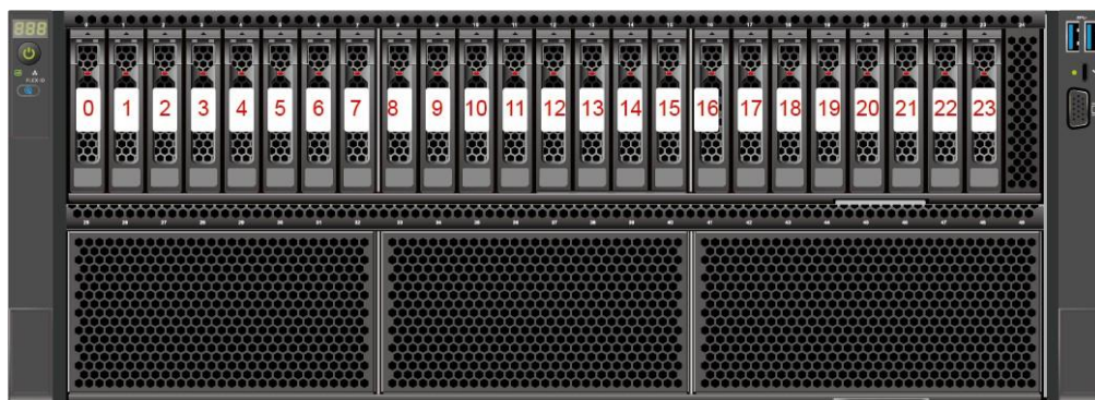
Figure 5-41 Drive numbering
